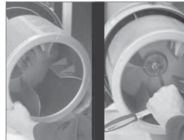
(15) Ensure bush (if your unit has one), shaft and drum hub are clean and free from debris before re-fitting the drum. If your unit includes a drum bush, tighten to 20Nm, if it includes taper collar(s), tighten bolt to 8Nm.
