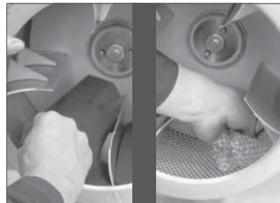
(5) Remove old drum pads, clean inside of drum and inspect drum for signs of damage. IMPORTANT! Damaged drums should be replaced.
