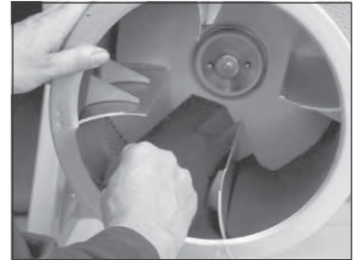
(6) Remove old drum pads.
