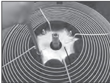
(14) IMPORTANT! Fit new motor mounting nuts & tighten (5Nm S Series or 8Nm FX Series).
