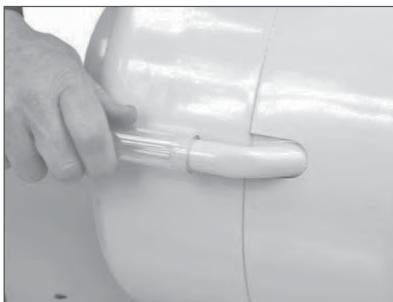
(7) Fit oil return tube and position tube to drain oil back to machine enclosure, sump or collection vessel.
